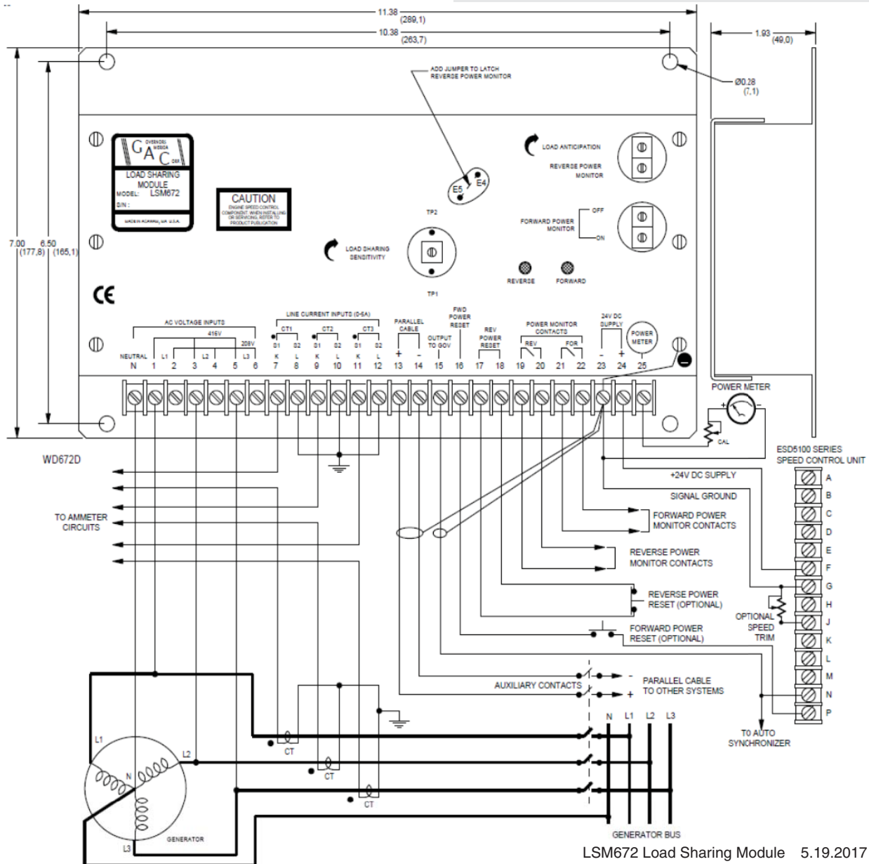
DIAGRAM 1: SYSTEM WIRING AND OUTLINE
