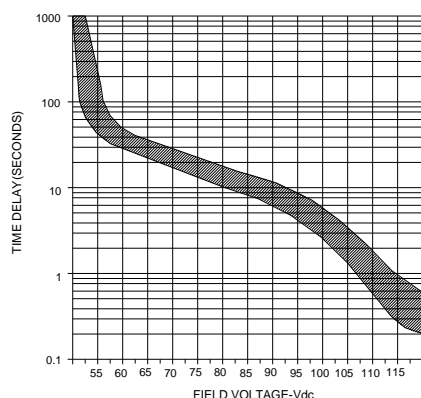
Figure 2 Typical Time Delay Characteristic Curve
