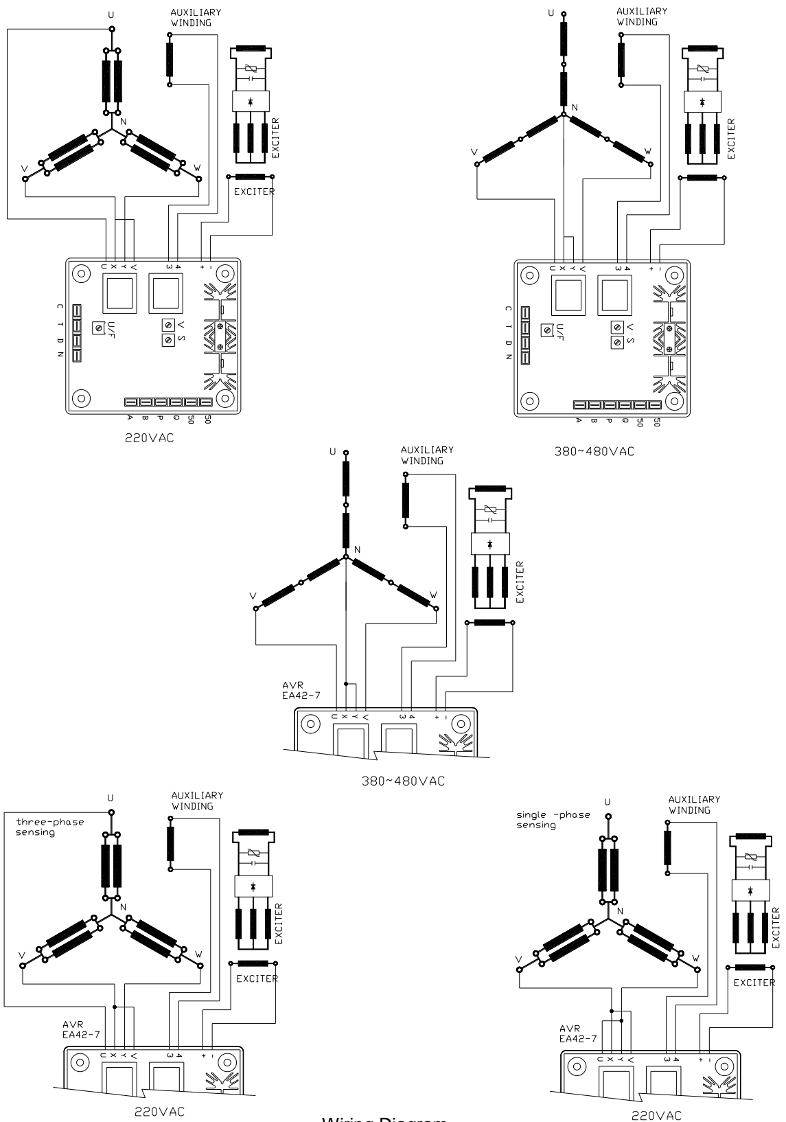
Wiring Diagram Figure 5
