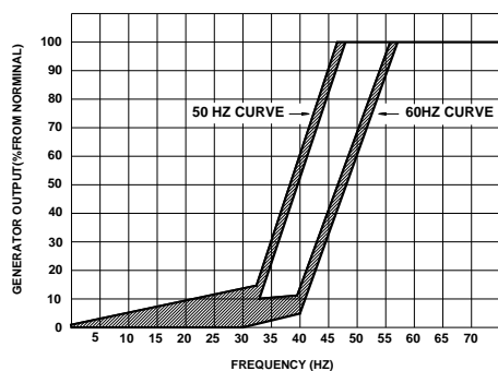
Figure 1 Frequency Compensation Curves
