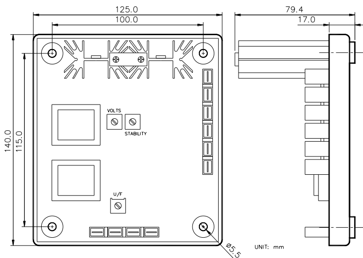
Outline Drawing Figure 3
