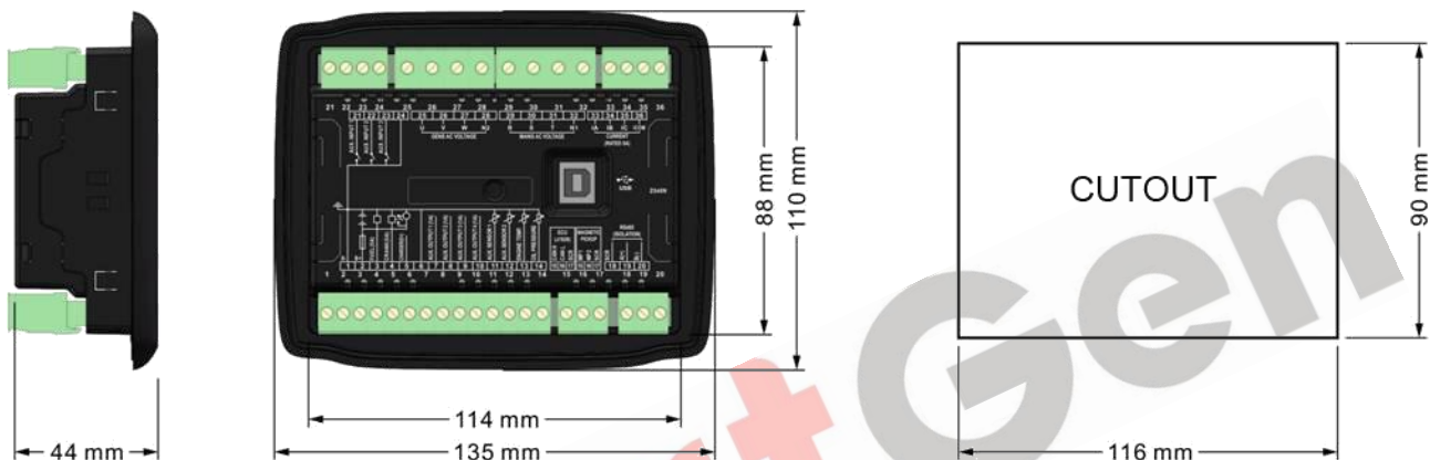
Fig.11 - Overall Dimensions and Cutout
