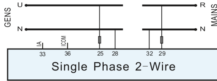
Fig.9 - Single Phase 2-Wire Connection Diagram
